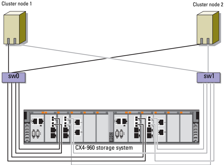
Figure 2-2. Cabling in a Dell/EMC SAN-Attached Fibre Channel Cluster
