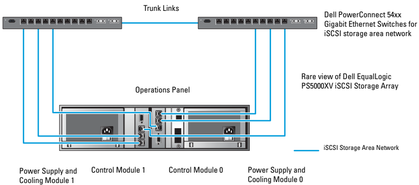
Figure 5-1. Recommended Network Configuration
