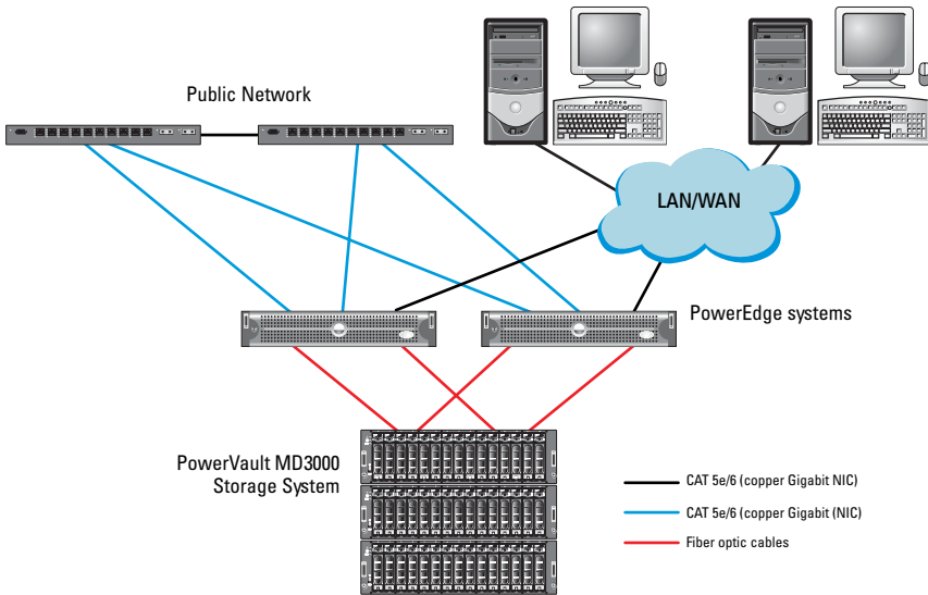
Figure 3-1. Cabling the Serial-Attached SCSI (SAS) Cluster and Dell PowerVault MD3000
